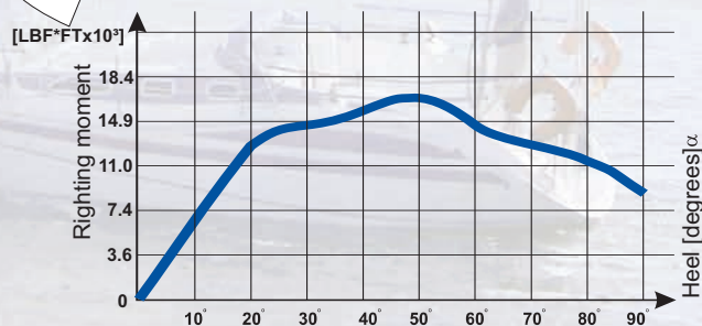
Righting moment curve
